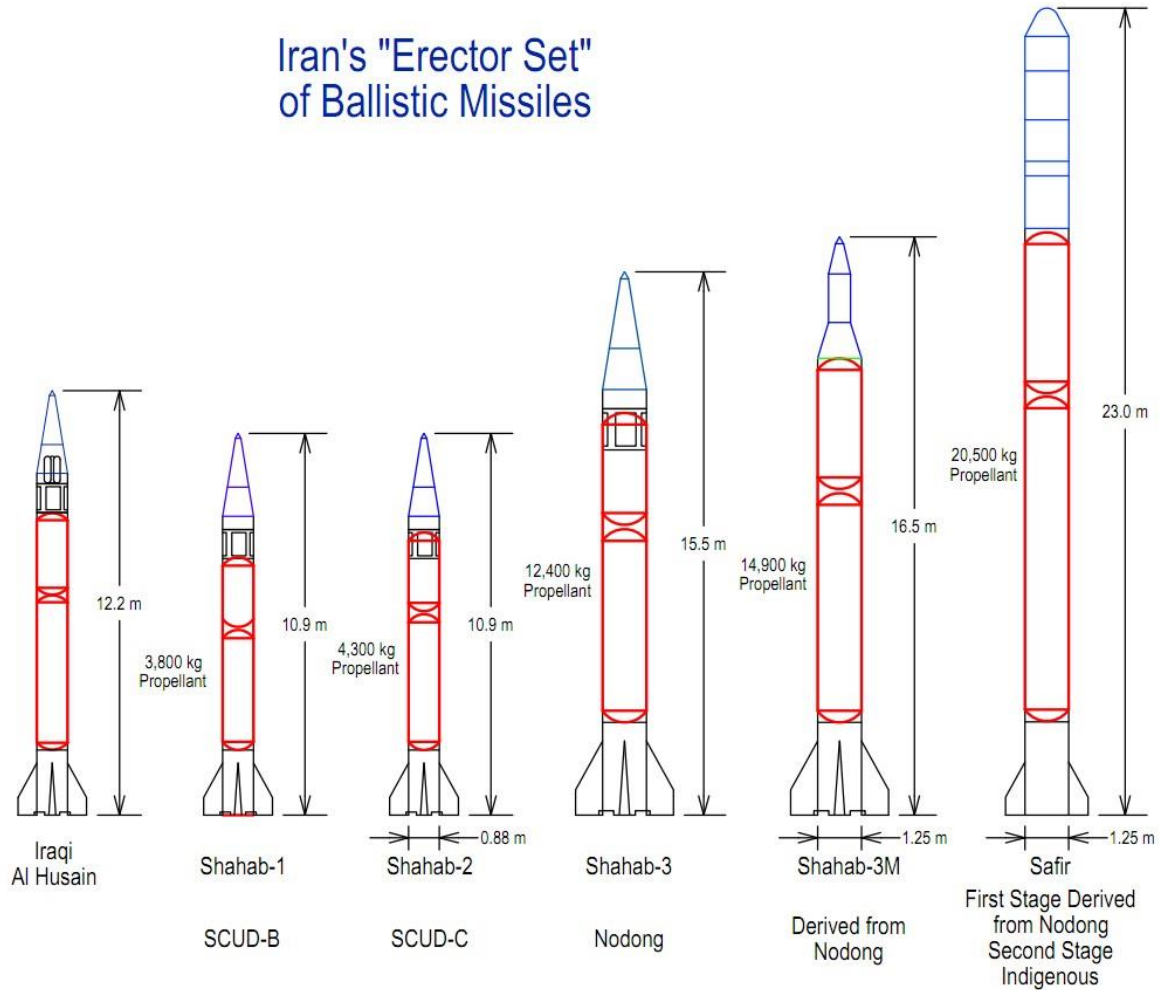
Figure 16: Iran’s “Erector Set” of Ballistic Missiles
