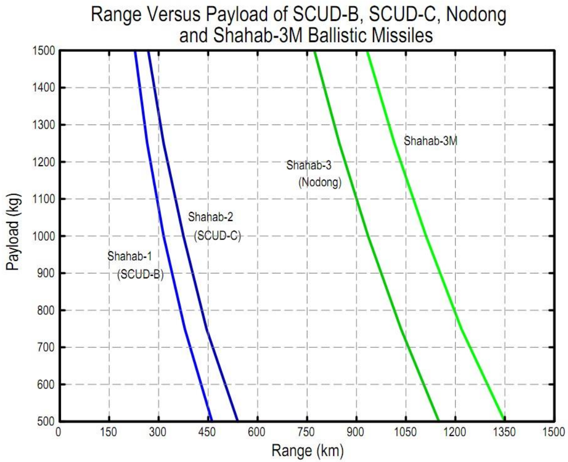
Figure 22: Range-Payload Relationship for Active Iranian Missiles - Part I
