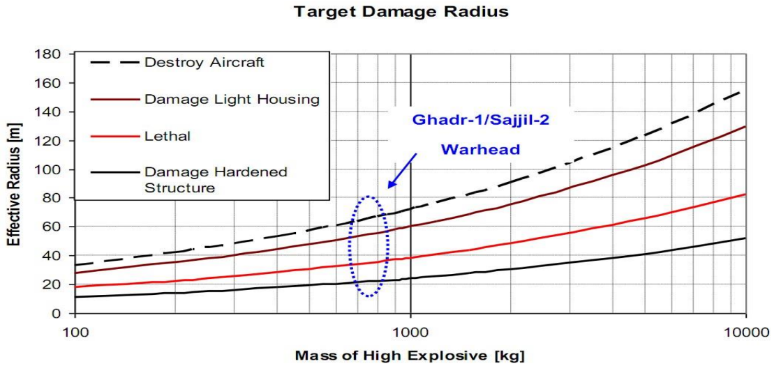
Figure 23: Estimate of Sejji Lethality Against Soft Targets
